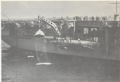
With the mock module in position to be swung over on Bennington's number three elevator (above), the recovery is complete, and the B & A Crane proceeds to lower it back into the water to give the USS Carpenter (DD-825), the secondary recovery ship, a trial run.
