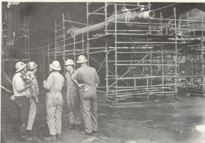
Above--Runout tests confirmed the part inboard shaft was bent. Yardworkers in foreground discuss its removal.
